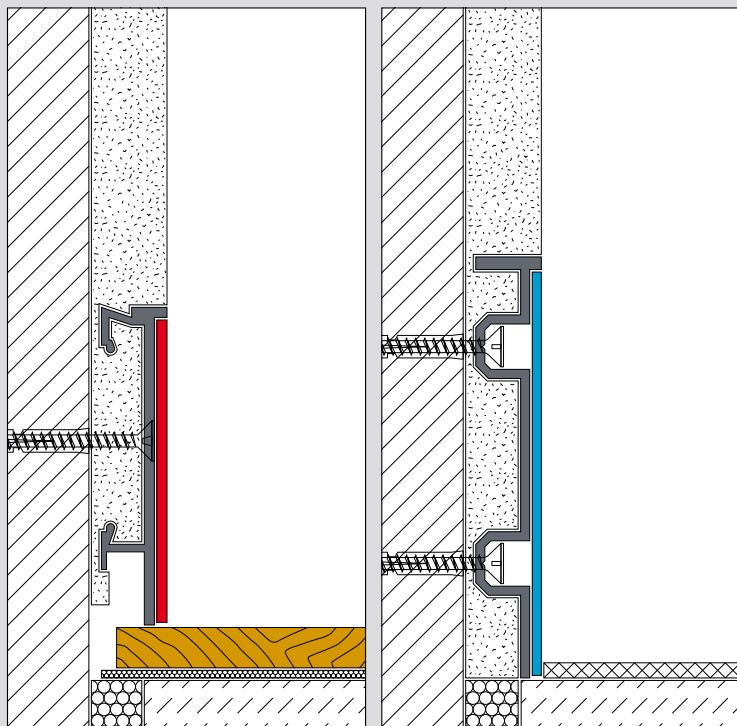
C63-13-BE2-PB in Profilkombination i60-2-ELO
