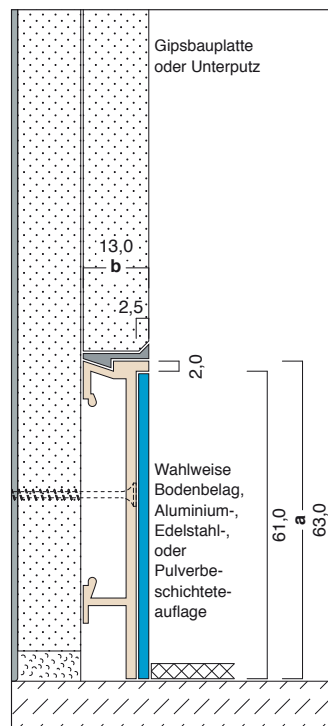
C22-E 63,0 x 13,0 mm
