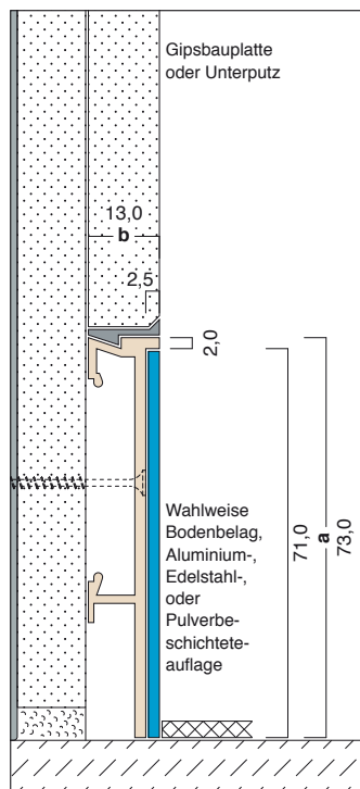
C23-E 73,0 x 13,0 mm
