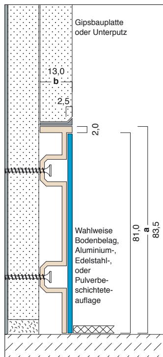
C12/U-E 82,5 x 13,0 mm
