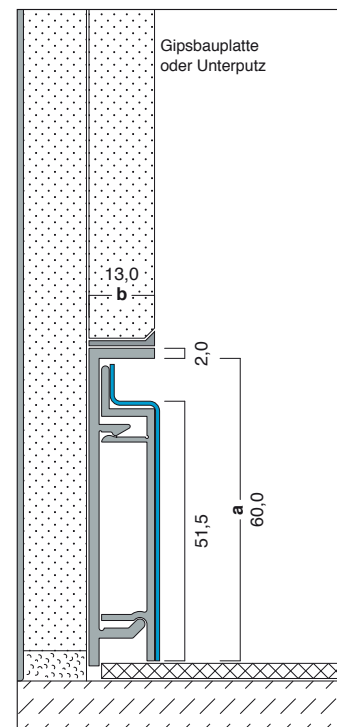
X60/U10-E 62,0 x 13,0 mm
