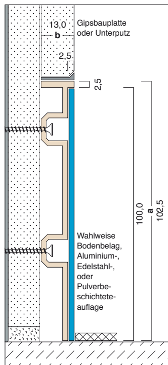
C8/U-E 102,5 x 13,0 mm
