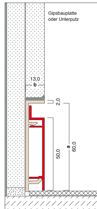
X60/U10 62,0 x 13,0 mm
