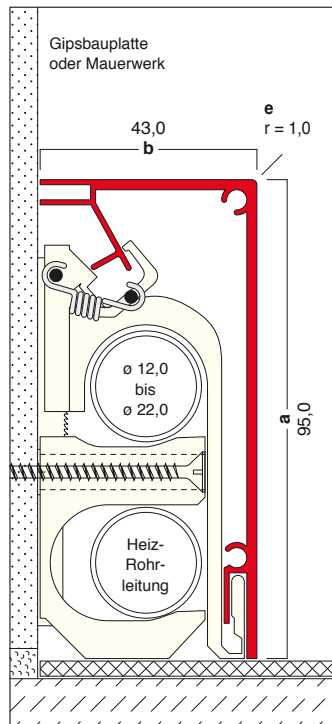
K2 95,0 x 43,0 mm
