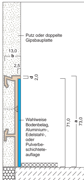
C23-E 73,0 x 13,0 mm
