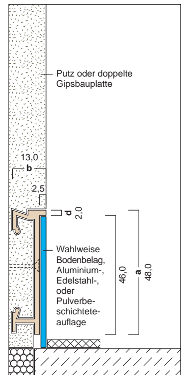
C21-E 48,0 x 13,0 mm
