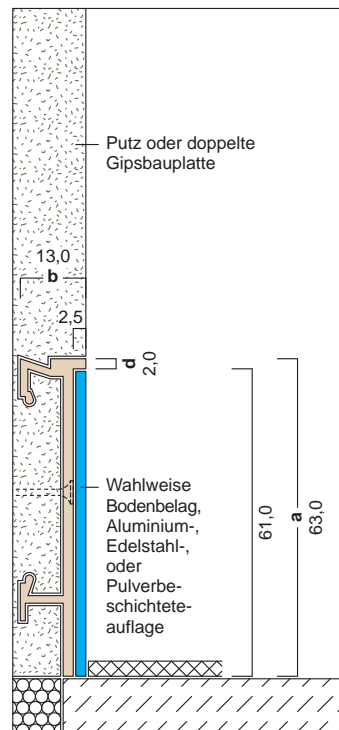
C22-E 63,0 x 13,0 mm
