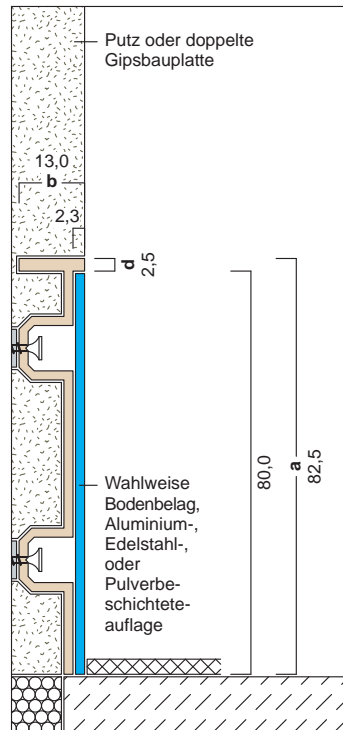
C12/U-E 82,5 x 13,0 mm
